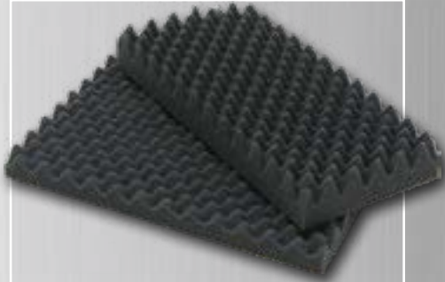
Noppenschaumplatte Stärke Best. Nr. egg-foam sheet thickness Order No. 1000 x 1000 mm 15 mm 3.830.9 30 mm 3.832.9 50 mm 3.834.9
